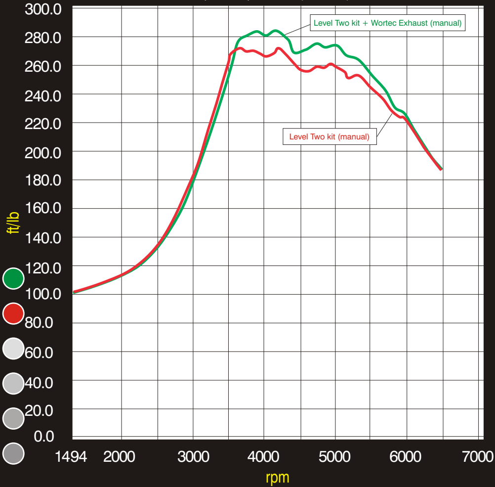
Wheel Torque Graph 944T (manual) - L2 kit
