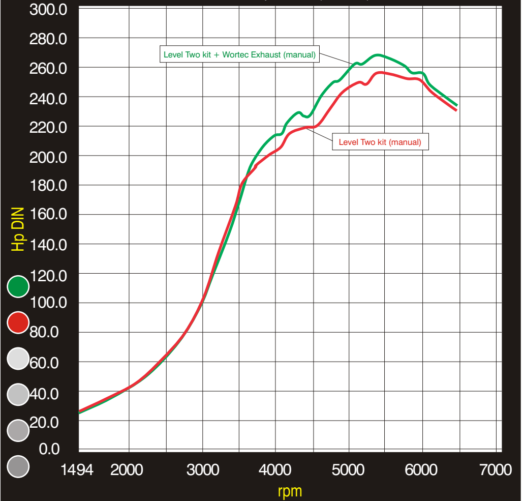
Wheel Power Graph 944T (manual) - L2 kit
