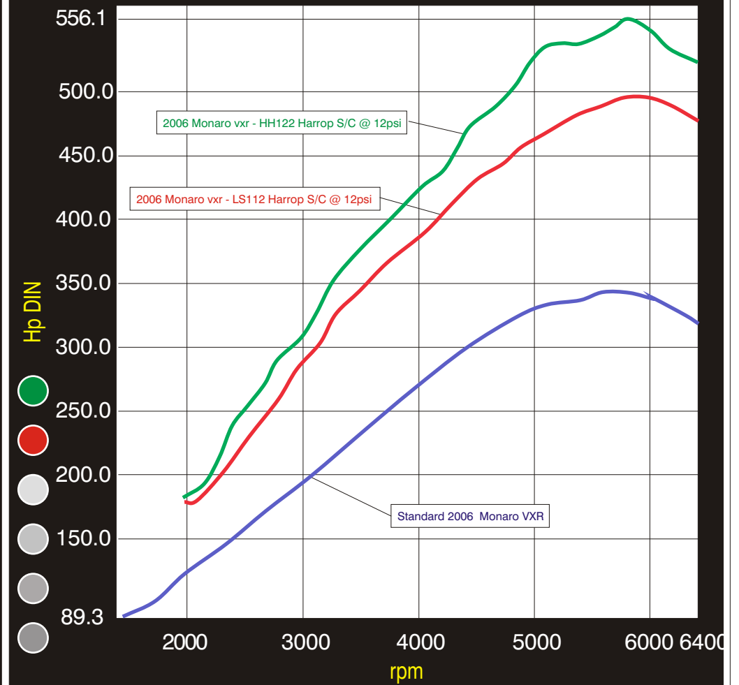
Hub Power Graph 2006 Monaro VXR S/C @ 12psi
