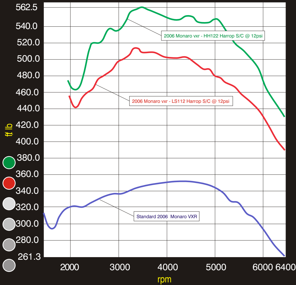
Hub Torque Graph 2006 Monaro VXR S/C @ 12psi
