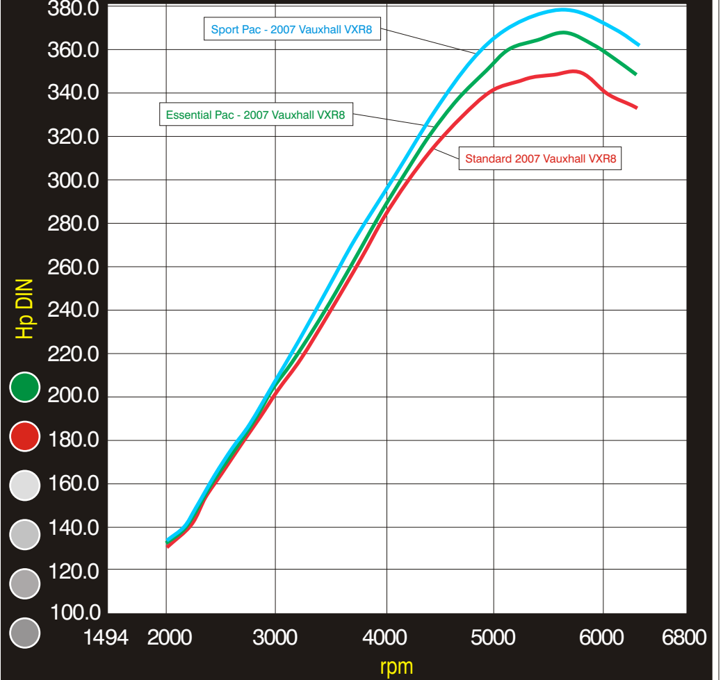
Hub Power Graph 2007 Vauxhall VXR8 - Essential/Sport pac
