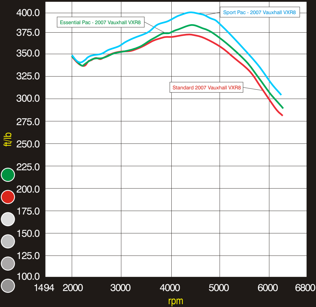
Hub Torque Graph 2007 Vauxhall VXR8 - Essential/Sport pac
