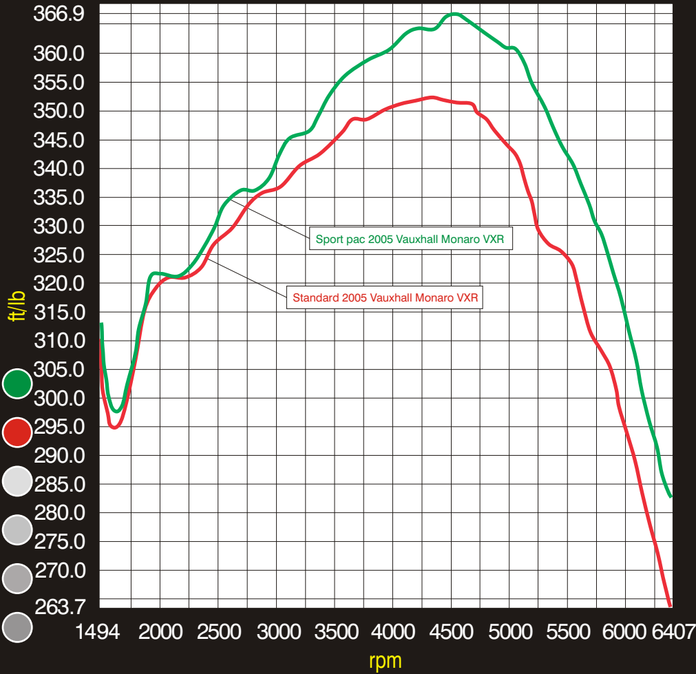
Hub Torque Graph 2005 Vauxhall Monaro VXR - Sport Pac
