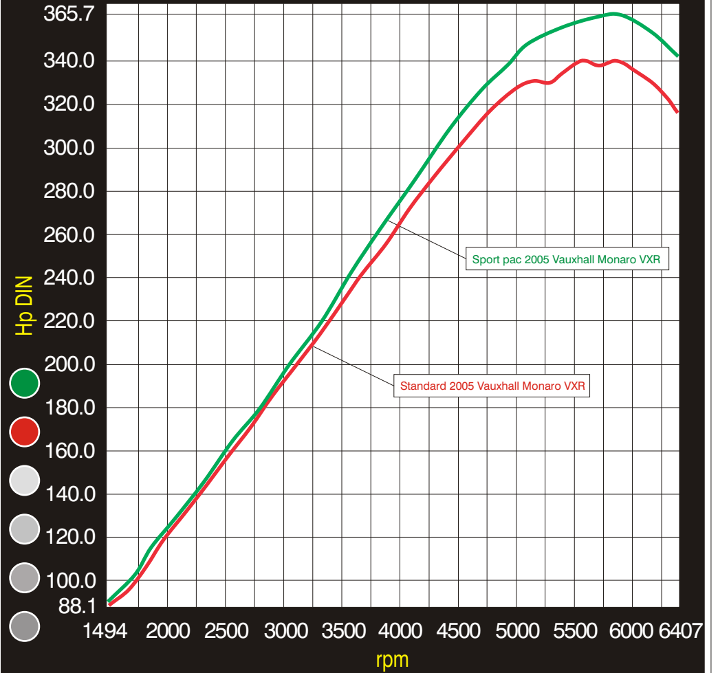
Hub Power Graph 2005 Vauxhall Monaro VXR- Sport Pac
