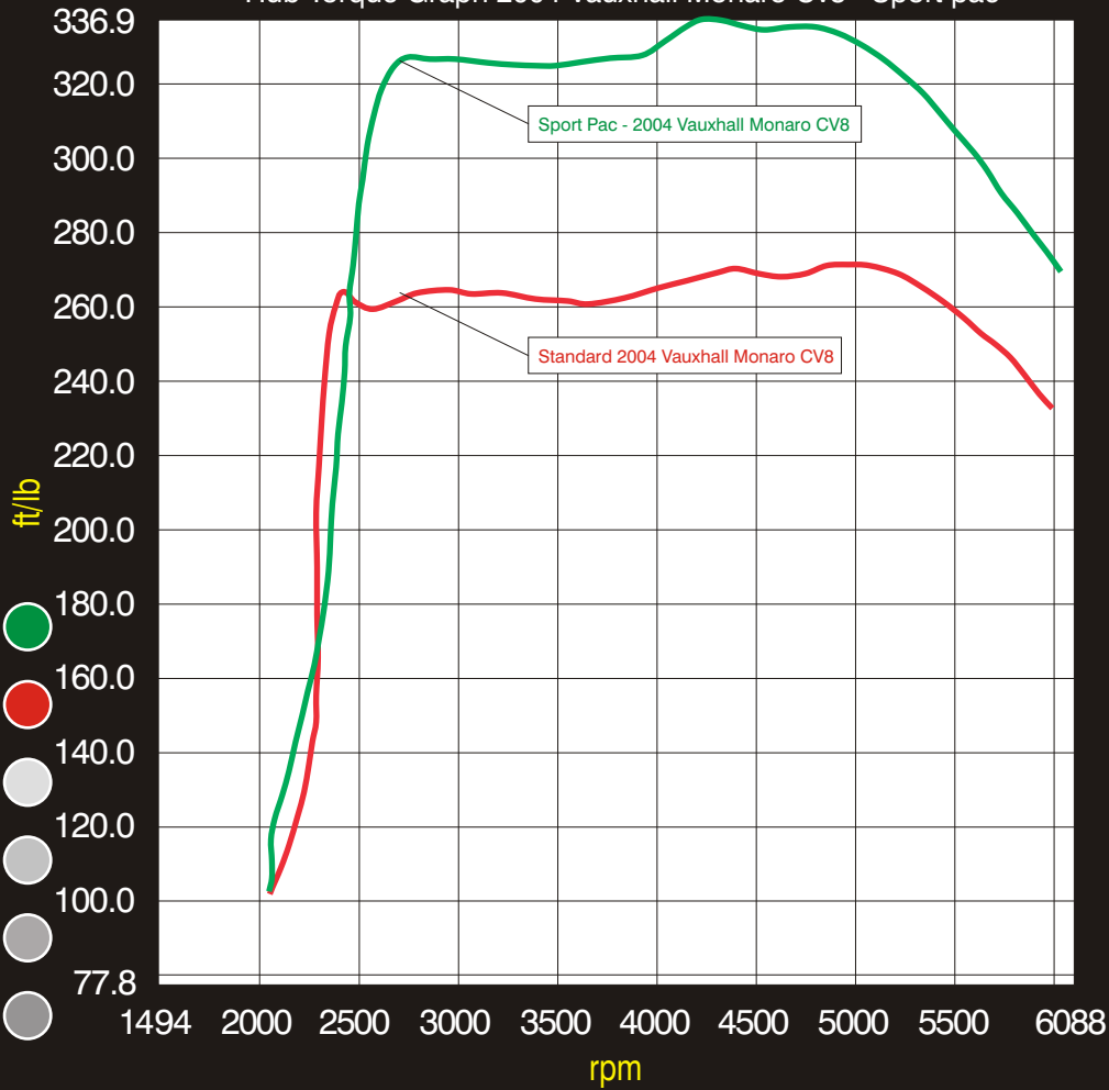
Hub Torque Graph 2004 Vauxhall Monaro Cv8 - Sport pac
