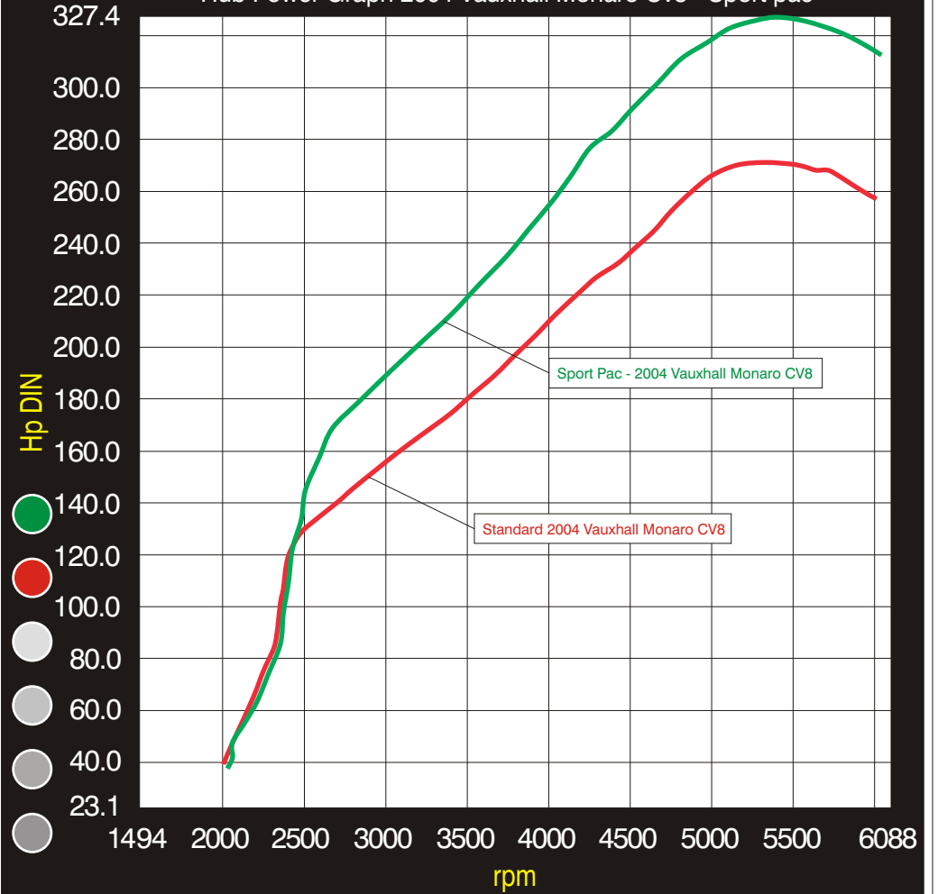
Hub Power Graph 2004 Vauxhall Monaro Cv8 - Sport pac
