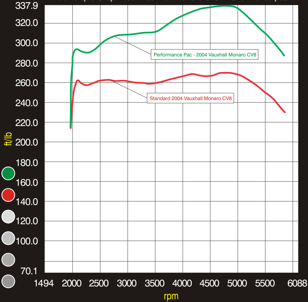
Hub Torque Graph 2004 Vauxhall Monaro Cv8 - Performance pac
