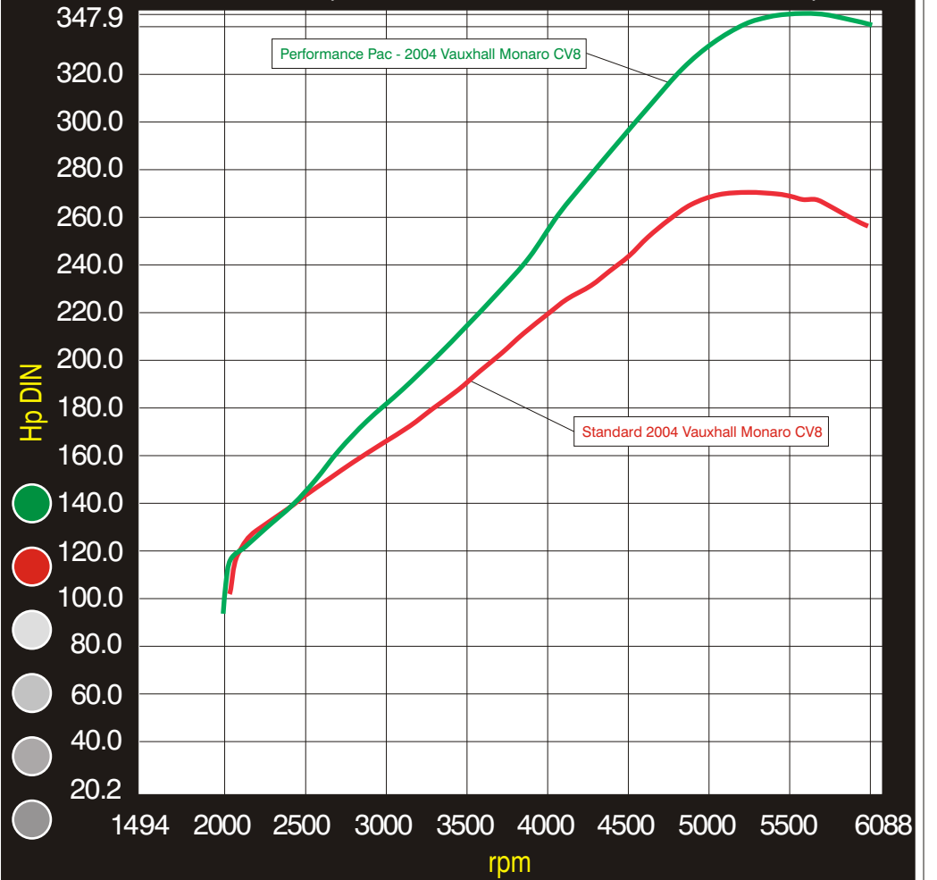
Hub Power Graph 2004 Vauxhall Monaro Cv8 - Performance pac
